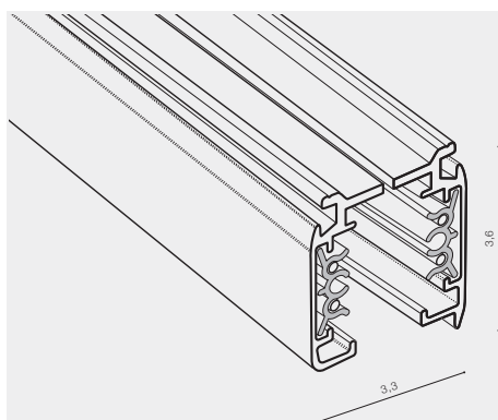
Example of the connection between track
