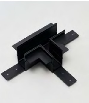
BETA TRACK MAGNETIC57 230V CONNECTOR T A GIPS2 Color/Code ● black ..... AZ6703
